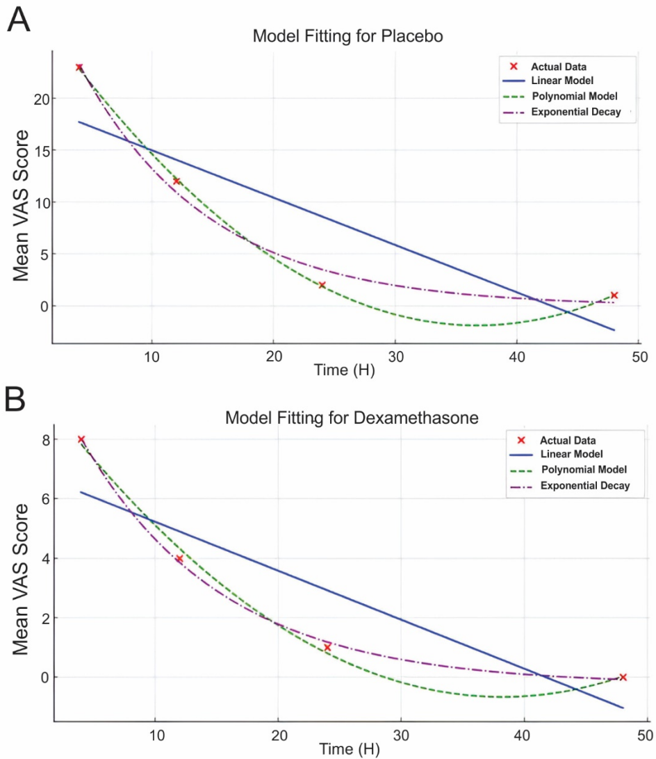
Figure S1: Exponential decay model for missing data imputation.
