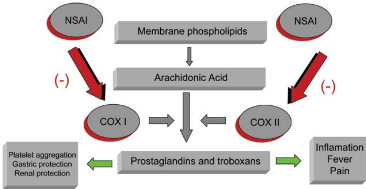
Fig. 2. Mechanism of action of NSAI.
