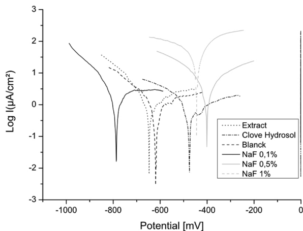
Fig. 1: Polarisation curves of NiTi in the different concentrations of NaF
