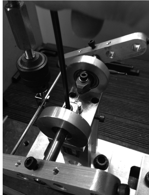
Fig. 3: The system attached by screws to avoid slipping of the set that could impair the results.
